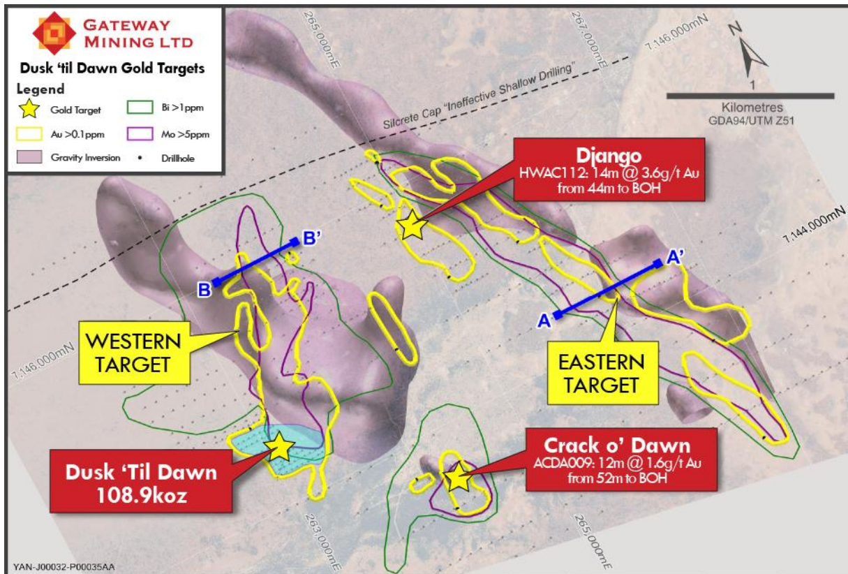
Figure 7. Shallow Au-Mo-Bi geochemical trends in relation to the 3D gravity inversion models.
