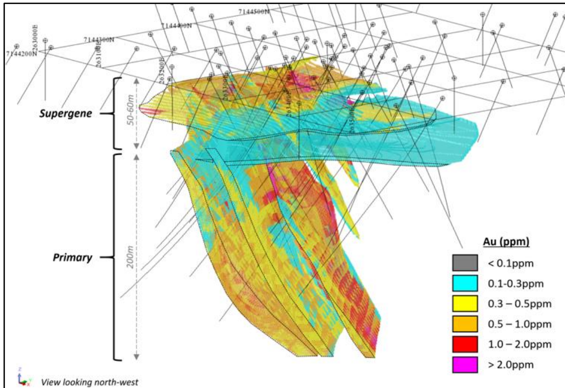
Figure 6. Dusk 'til Dawn 108.9koz Resource Model coloured by Au ppm.
